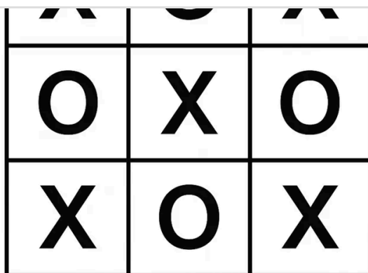
Tic-Tac-Toe
